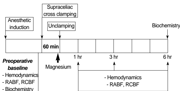
Fig. 1. Schematic diagram of the experimental protocol and data collection. RABF, renal artery blood flow; RCBF, renal cortical blood flow. Biochemistry include plasma renin activity, serum creatinine, Cystatin-C, and serum magnesium and calcium concentrations.
