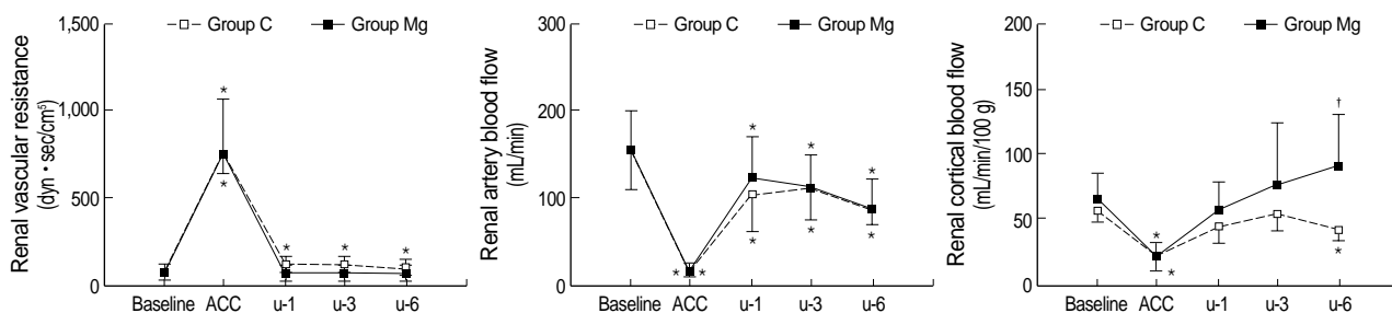
Fig. 2. Renal vascular resistance, renal artery blood flow, and renal cortical blood flow in anesthetized dogs after supraceliac aortic cross clamping and unclamping. ACC; supraceliac aortic cross clamping, U-1, 3, and 6=1, 3, and 6 hr after supraceliac aortic unclamping. * p < 0.05 versus baseline, † p < 0.05 versus control.
