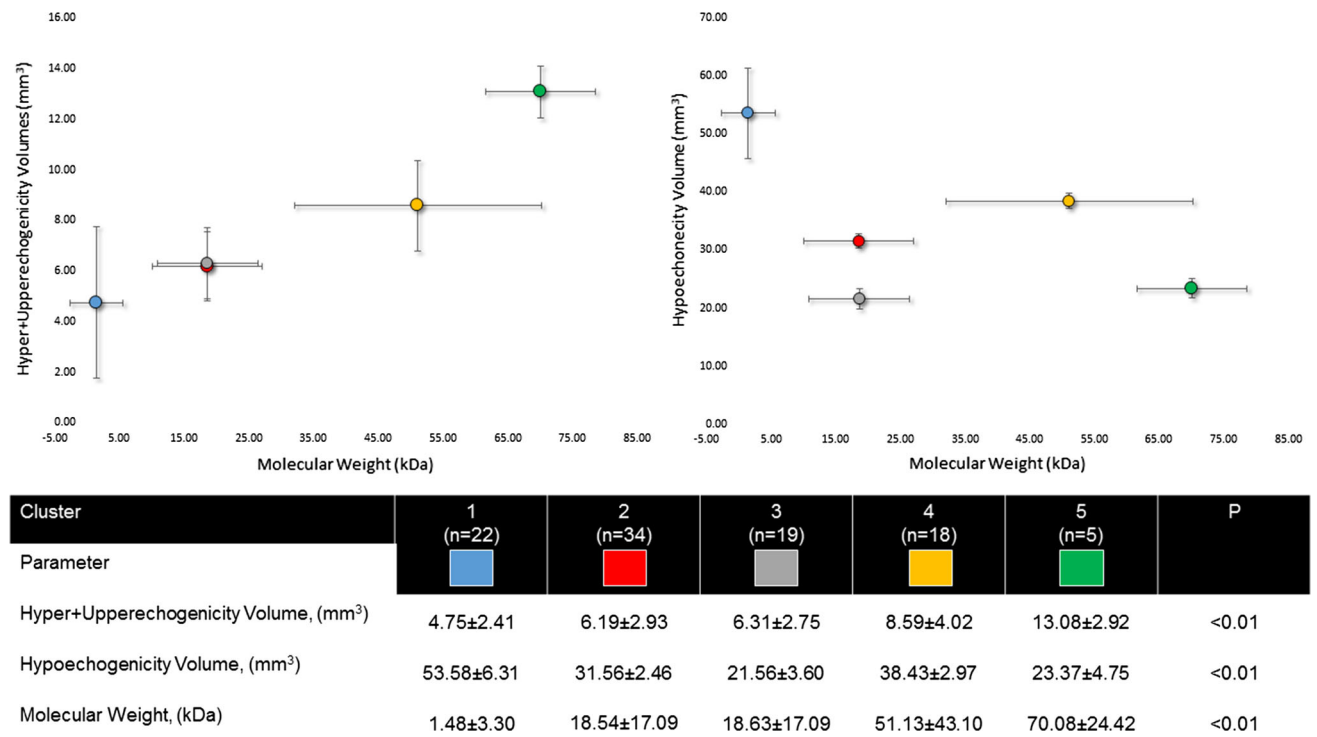
Fig. 5 A hierarchical cluster analysis labeled by animal was run for scaffold-vessel hyper + upperechogenicity and hypoechogenicity. Cluster 2 and 3 had similar hyper + upperechogenicity but statistically significant greater hypoechogenicity volumes in the cluster 2. Cluster 3 and 5 had similar hypoechogenicity but markedly higher
