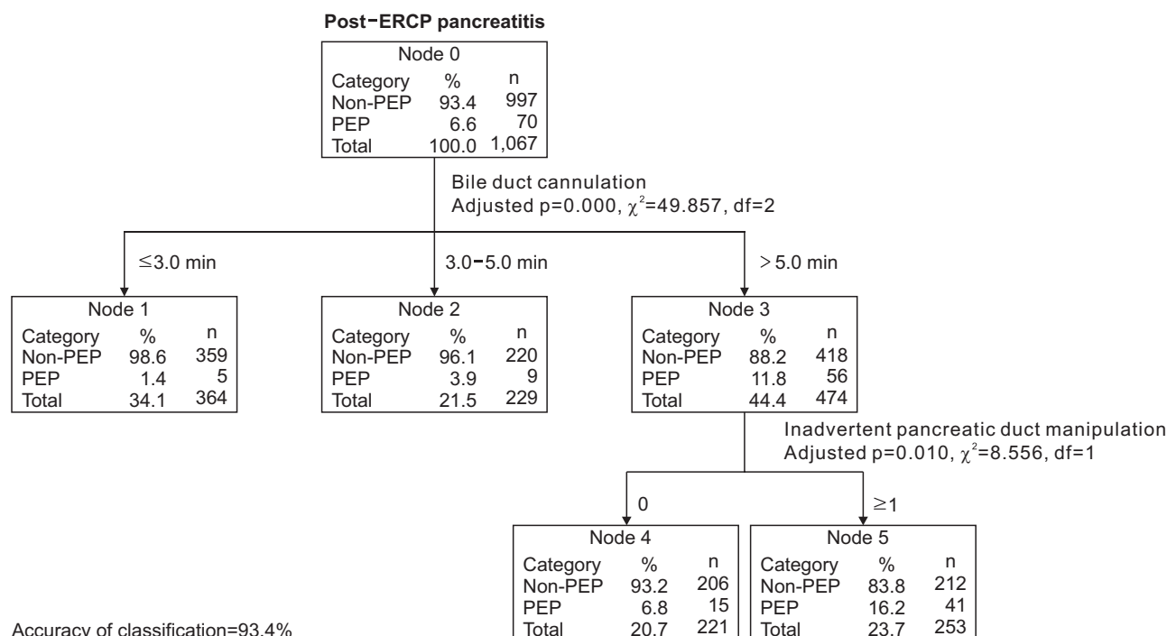
Fig. 1. A decision tree model for the prediction of post-ERCP pancreatitis generated by classification and regression tree analysis using our ERCP database.
