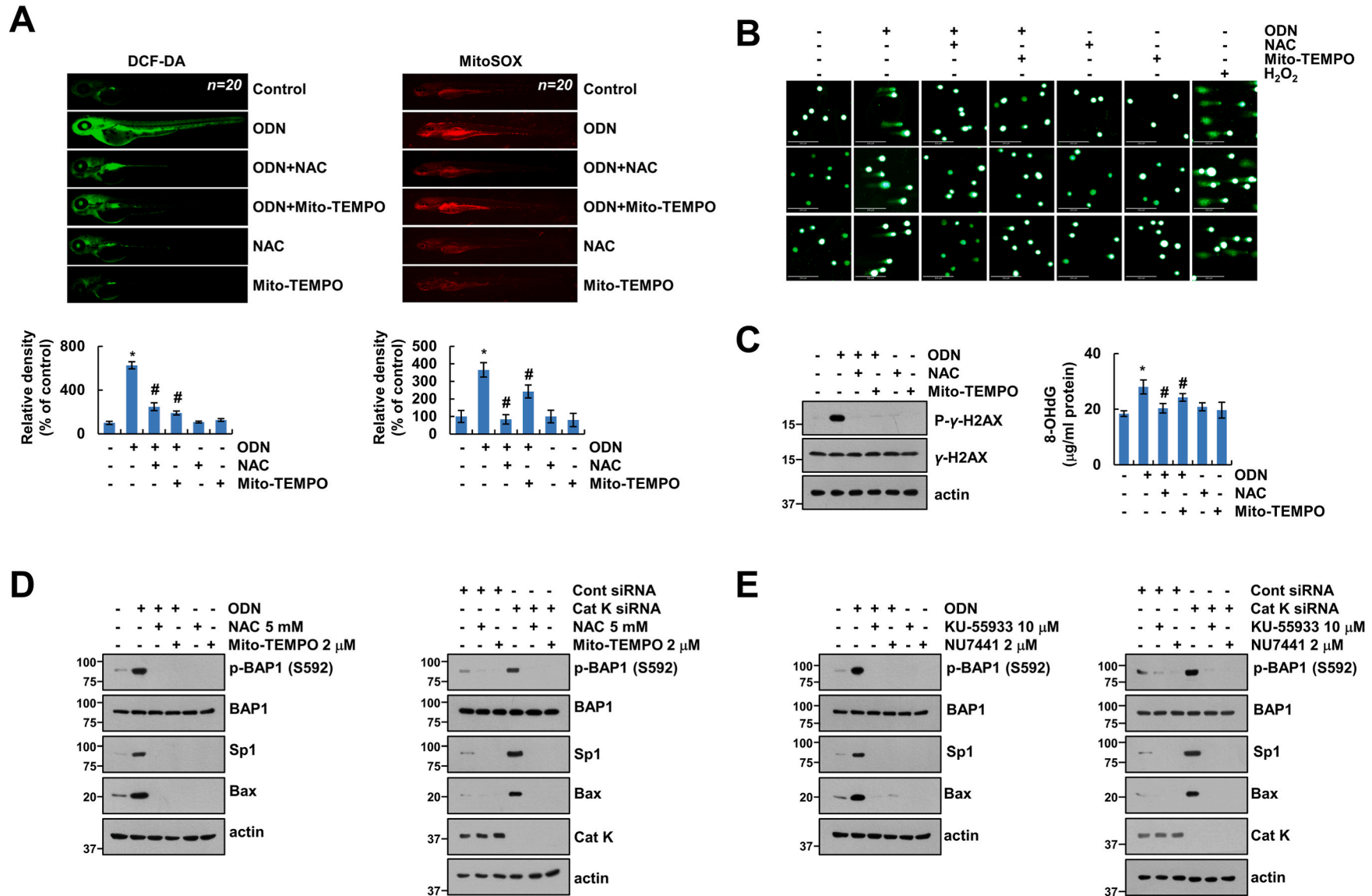
Fig. 9. ODN-induced mitochondrial ROS generation is involved in BAP1/Sp1/Bax activation. (A) Zebrafish larvae or (B, C) Caki-1 cells were pretreated with ROS scavengers (5 mM NAC and 2 \mu M Mito-TEMPO) for 1 h and then treated with 2 \mu M ODN for 24 h. ROS levels were observed under a fluorescence microscope after DCF-DA or MitoSOX staining (A). Representative images of the comet assay results were captured using a fluorescence microscope ( \times 200 ) (B). p- \gamma H2AX level was measured by western blotting, and the 8-OHdG level of the DNA samples of the cells was assessed (C). (D) Caki-1 cells were pretreated with ROS scavengers (5 mM NAC and 2 \mu M Mito-TEMPO) and then treated with 2 \mu M ODN or Cat K siRNA for 24 h. (E) Caki-1 cells were pretreated with 10 \mu M KU-55933 or 2 \mu M NU7441 or Cat K siRNA for 24 h. (C–E) Protein expression level was determined using western blotting. Values in the graphs (A, C) represent the mean \pm SD of three independent experiments. * p < 0.01 compared with control. # p < 0.01 compared with ODN treatment.
