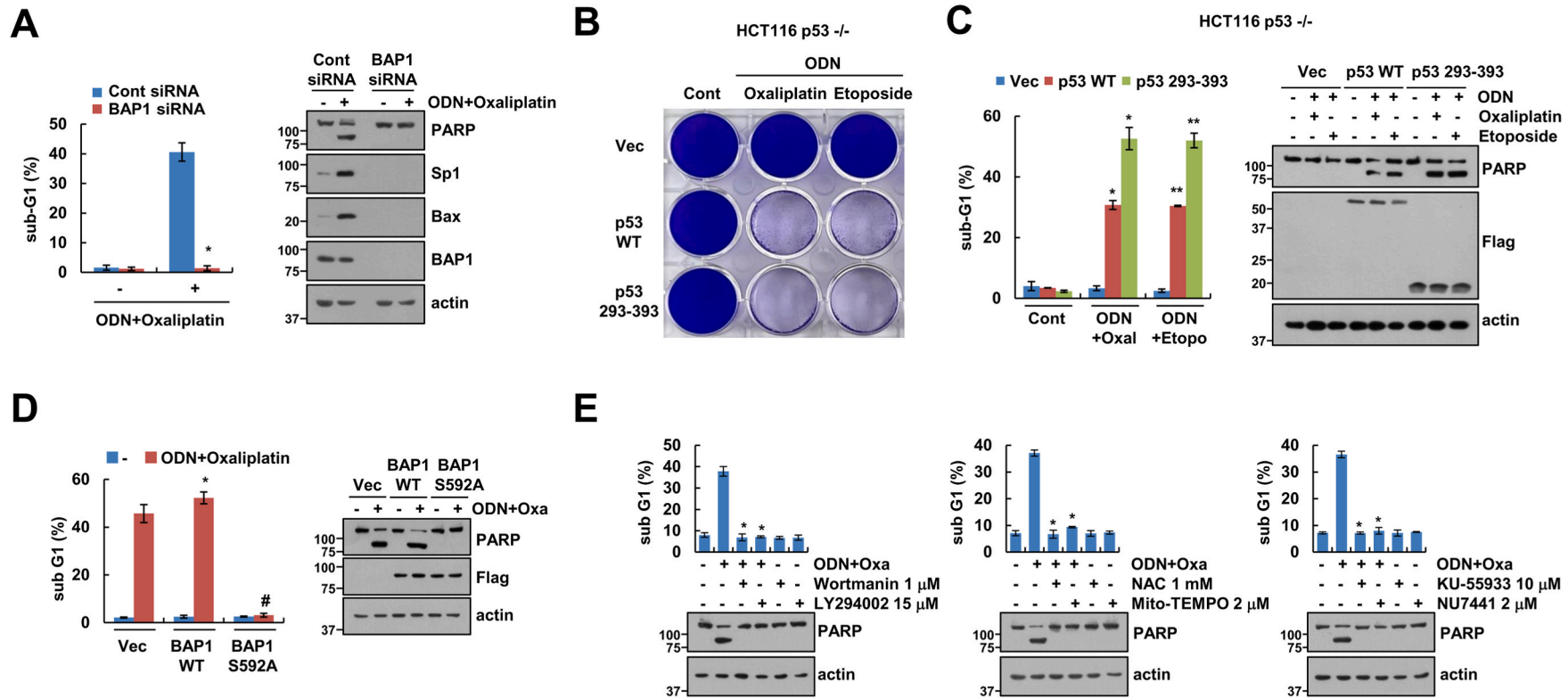
Fig. 10. Effect of BAP1 on ODN plus oxaliplatin-induced cancer cell death. (A) Caki-1 cells were transfected with control siRNA or BAP1 siRNA and treated with a combination of 2 \mu M ODN and 25 \mu M oxaliplatin for 24 h. (B, C) p53-null ( -/- ) HCT116 cells were transfected with the vector, WT p53, or p53 deletion mutant (293–393) and treated with a combination of 2 \mu M ODN and 25 \mu M oxaliplatin/3 \mu g/mL etoposide for 24 h. Colony formation was measured using crystal violet staining. (D) Caki-1 cells were transfected with vector, WT BAP1, or BAP1 mutant (S592A) and treated with a combination of 2 \mu M ODN and 25 \mu M oxaliplatin for 24 h. (E) Caki-1 cells were pretreated with various inhibitors (1 \mu M wortmannin, 15 \mu M LY294002, 5 mM NAC, 2 \mu M Mito-TEMPO, 10 \mu M KU-55933, or 2 \mu M NU7441) and treated with a combination of 2 \mu M ODN and 25 \mu M oxaliplatin for 24 h. Apoptosis and protein expression levels were measured using flow cytometry (A, C–D) and western blotting (A, C–E). Values in the graphs (A, C–E) represent the mean \pm SD of three independent experiments. * p < 0.01 compared with ODN plus oxaliplatin in the vector. ** p < 0.01 compared with ODN plus etoposide in the vector. # p < 0.01 compared with ODN plus oxaliplatin in WT BAP1-transfected cells. (For interpretation of the references to colour in this figure legend, the reader is referred to the Web version of this article.)
