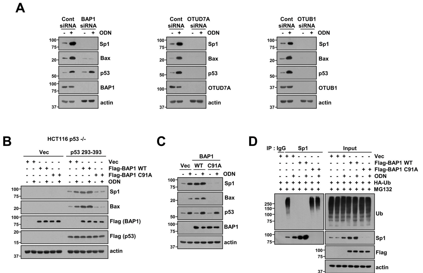
Fig. 6. BAP1 decreases Sp1 ubiquitination by the C-terminal domain of p53. (A) Caki-1 cells were transfected with control siRNA or 3 DUB (BAP1, OTUD7A, and OTUB1) siRNAs and treated with 2 \mu M ODN for 24 h. (B) p53-null (–/–) HCT116 cells were co-transfected with the vector or p53 deletion mutant (293–393), together with WT BAP or BAP mutant (C91A), and treated with 2 \mu M ODN for 24 h. (C) Caki-1 cells were transfected with the vector, WT BAP, or BAP mutant (C91A) and treated with 2 \mu M ODN for 24 h. (D) Caki-1 cells were co-transfected with the vector, WT BAP, or BAP mutant (C91A) and HA-ubiquitin (HA-Ub), and treated with 0.5 \mu M MG132 for 12 h to analyze Sp1 ubiquitination. Immunoprecipitation was performed using an anti-Sp1 antibody. (A–D) Protein expression level was determined using western blotting.
